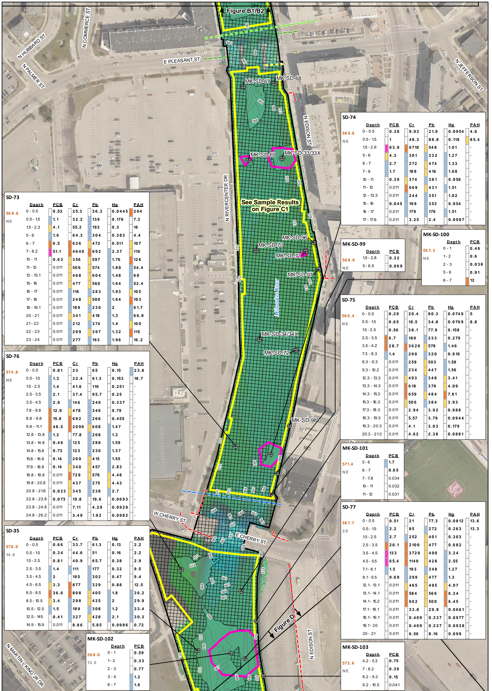
Figure 7-1C2 Recommended Remedial Alternative 3A Milwaukee River Downtown Reach Milwaukee Estuary Area of Concern Milwaukee, Wisconsin
