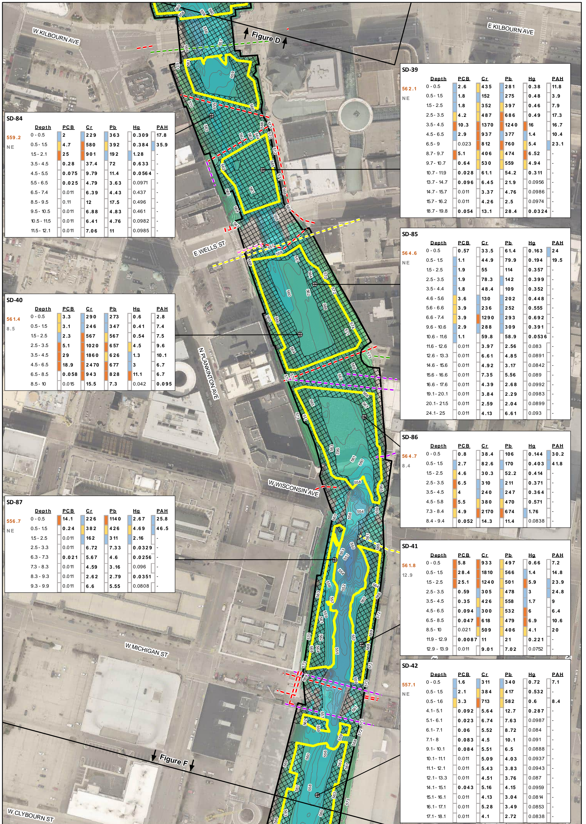
Figure 7-1E Recommended Remedial Alternative 3A Milwaukee River Downtown Reach Milwaukee Estuary Area of Concern Milwaukee, Wisconsin
