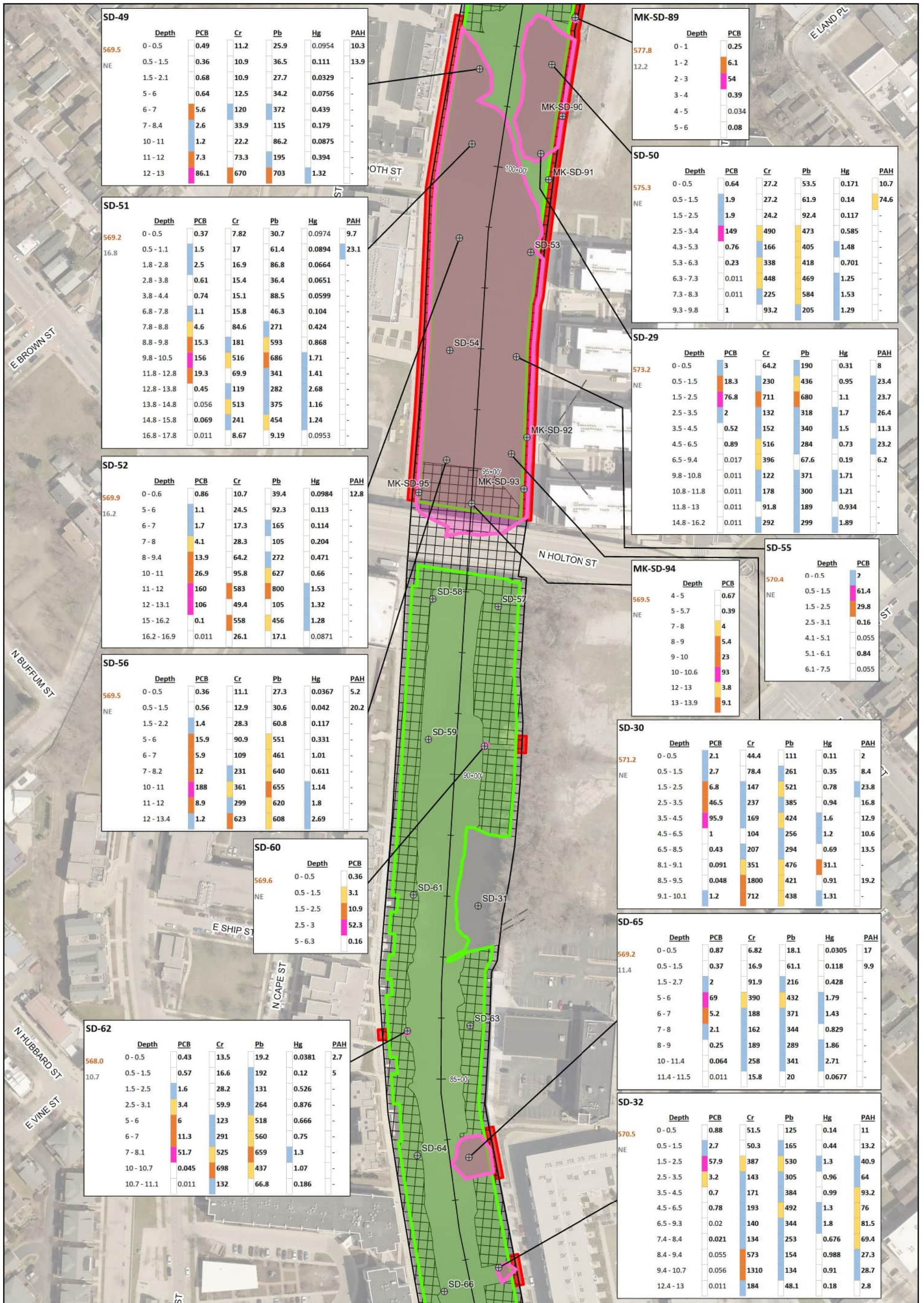
Figure 5-2B Downtown Reach - Alternative 3 Conceptual Layout Milwaukee Estuary Area of Concern Milwaukee, Wisconsin
