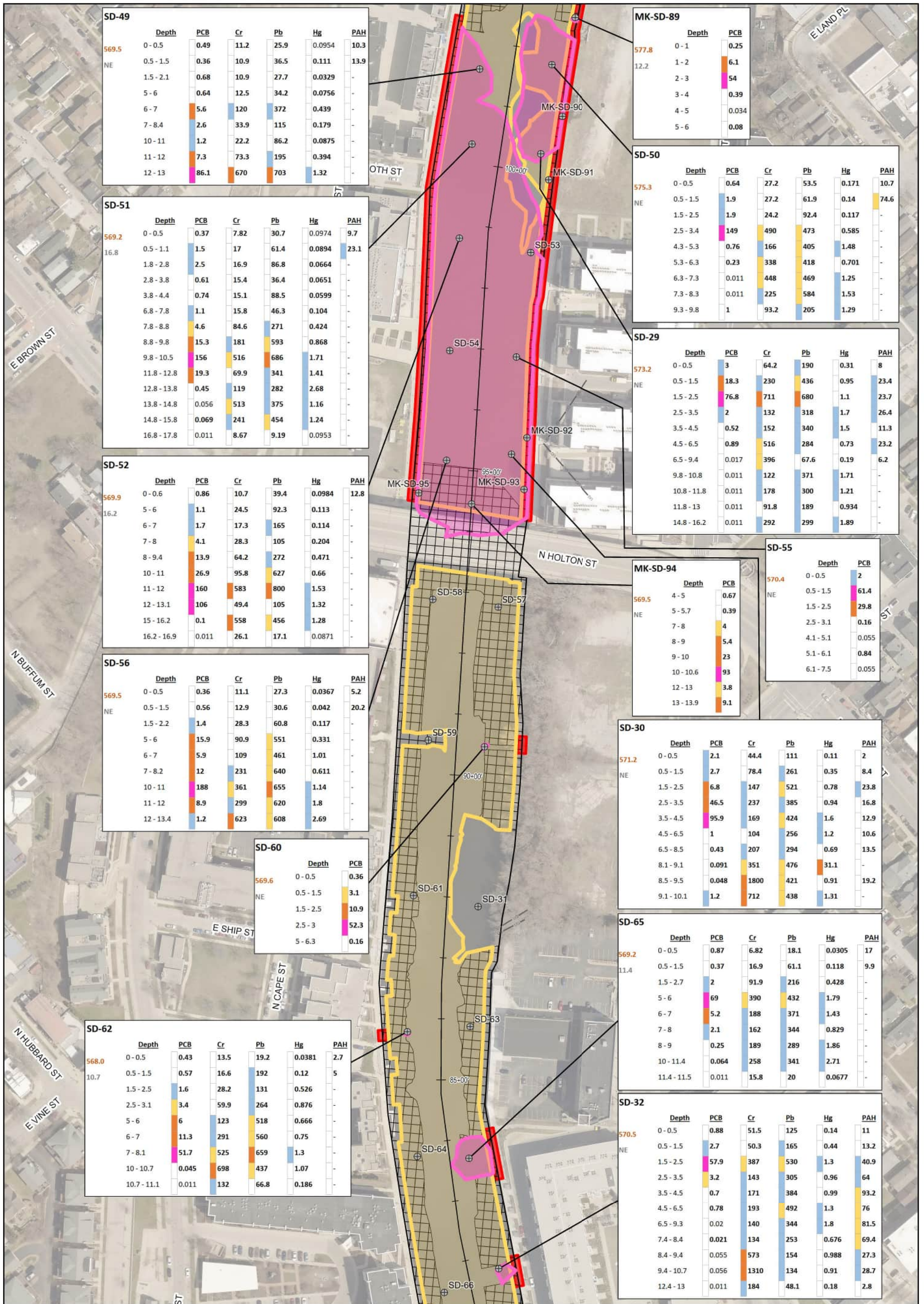
Figure 5-4B Downtown Reach - Alternative 4 Conceptual Layout Milwaukee Estuary Area of Concern Milwaukee, Wisconsin
