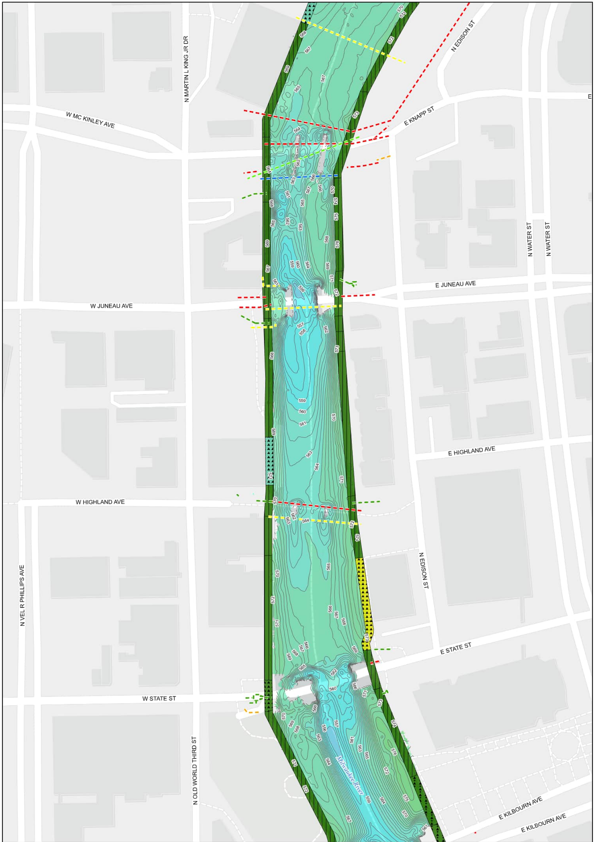
Figure 1-2D Site Features Milwaukee River Downtown Reach Milwaukee Estuary Area of Concern Milwaukee, Wisconsin
