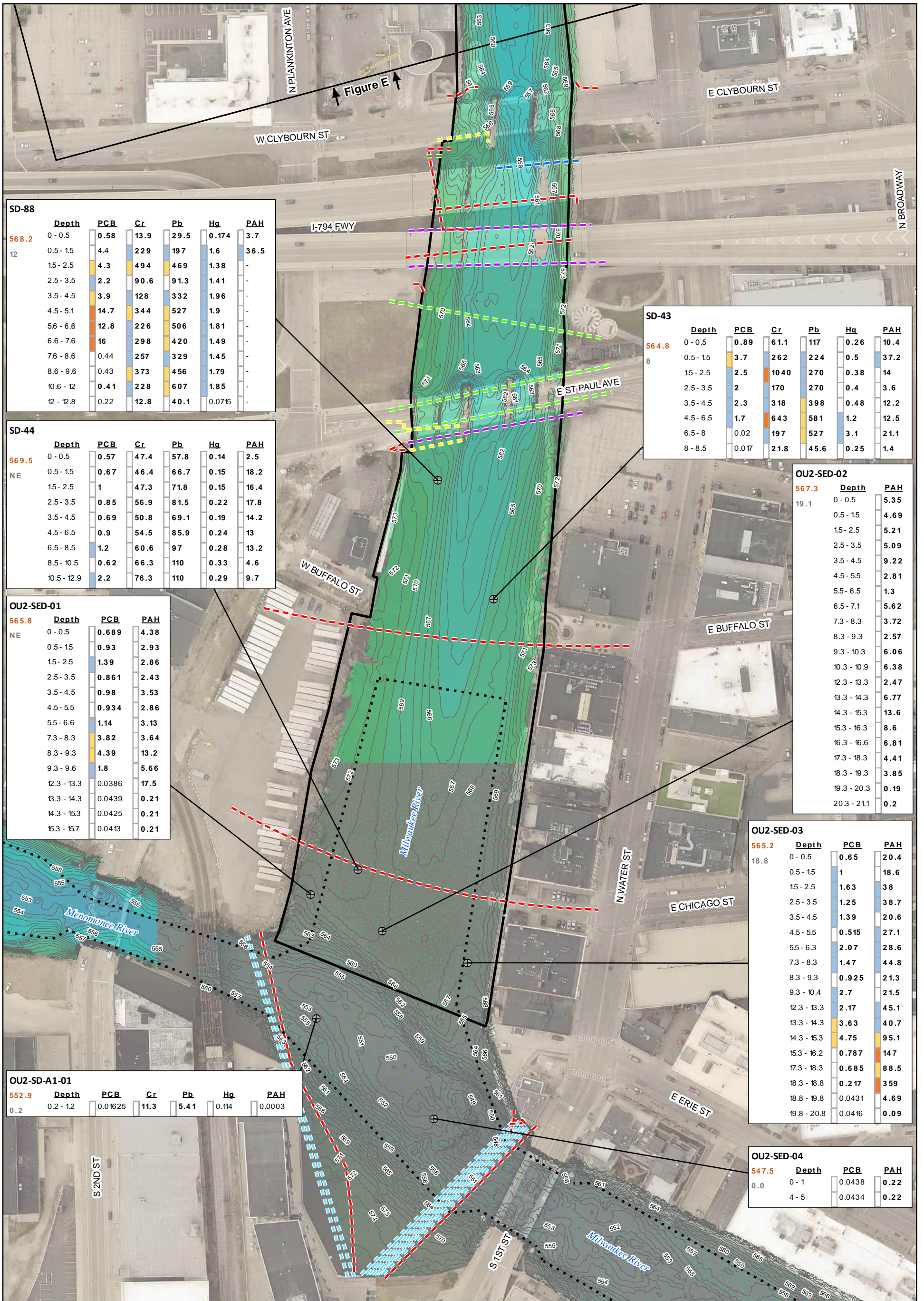
Figure 2-3F Recommended Remedial Alternative Milwaukee River Downtown Reach Milwaukee Estuary Area of Concern Milwaukee, Wisconsin
